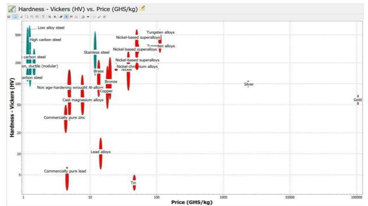
Figure 1: CES Graph
